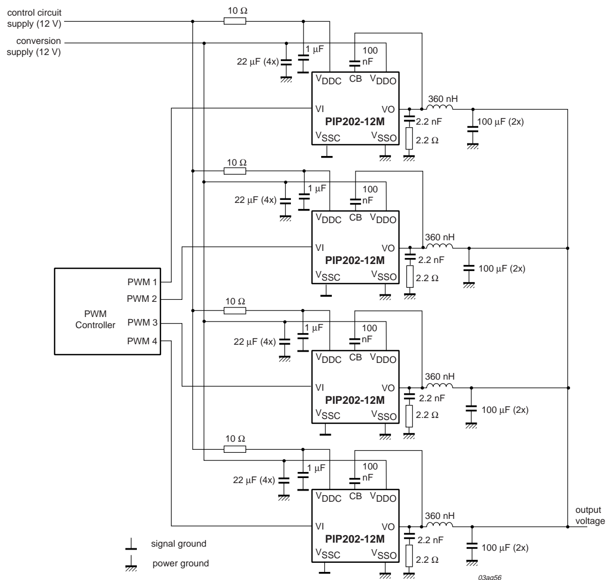
Fig 11. Typical application circuit using the PIP202-12M in a four-phase converter.
