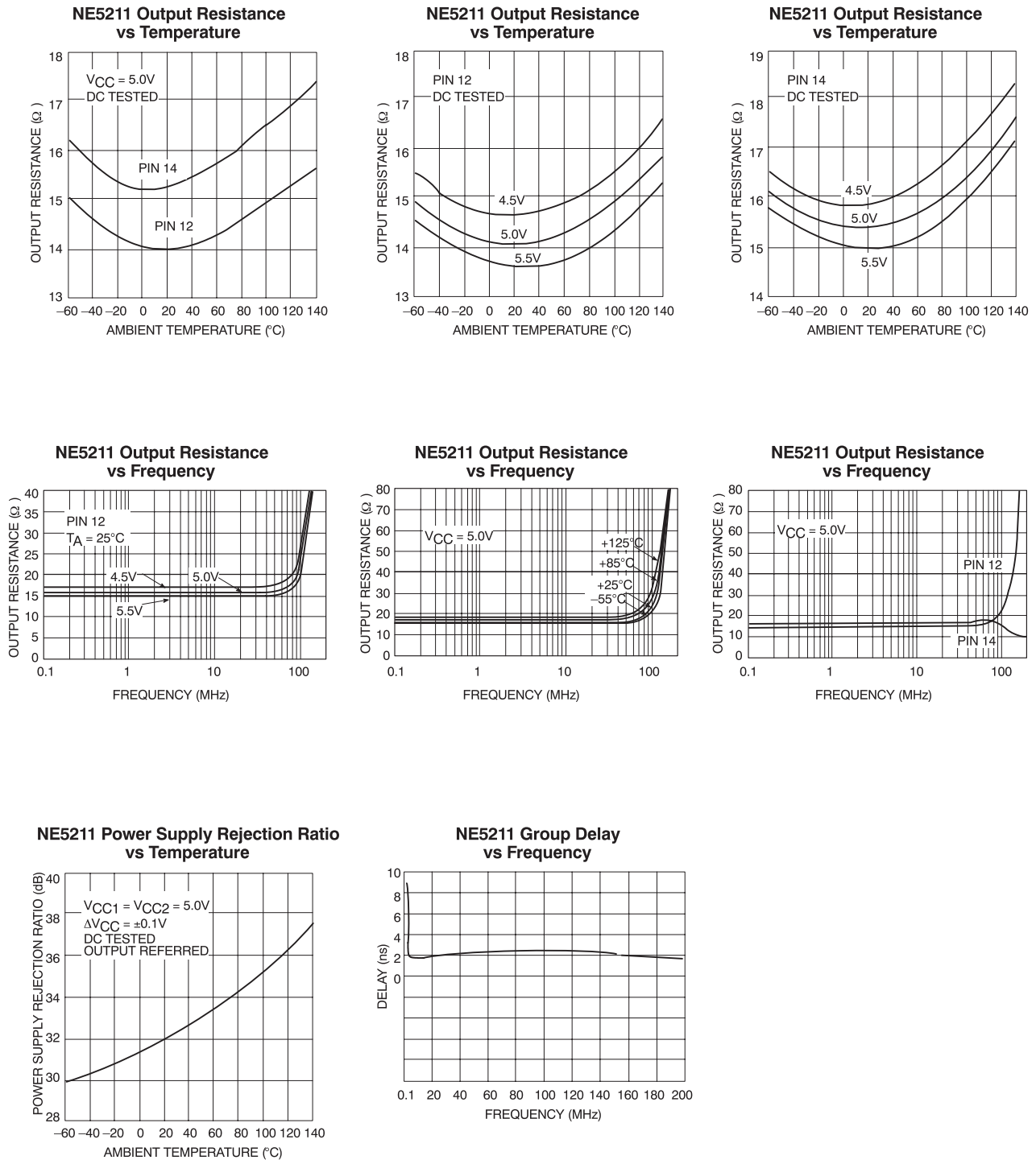
Fig 9. Typical performance characteristics. (cont.)
