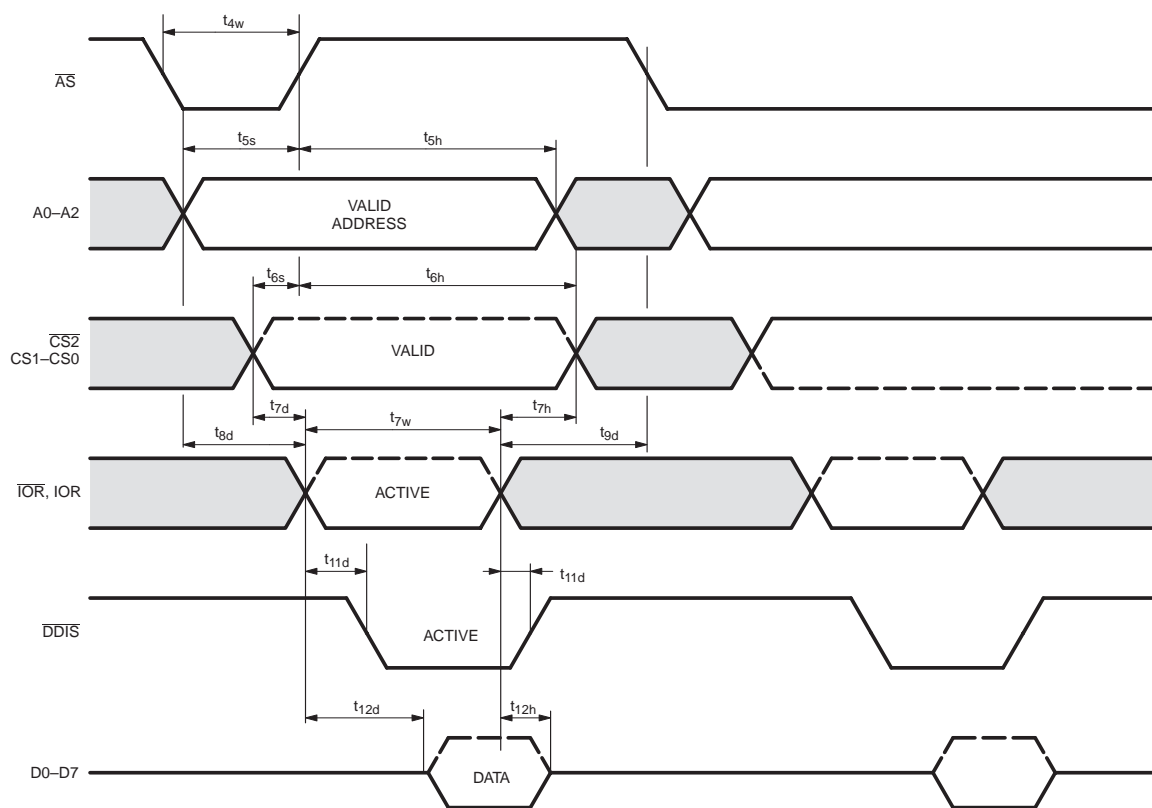
Fig 6. General read timing when using \overline{\text{AS}} signal.
