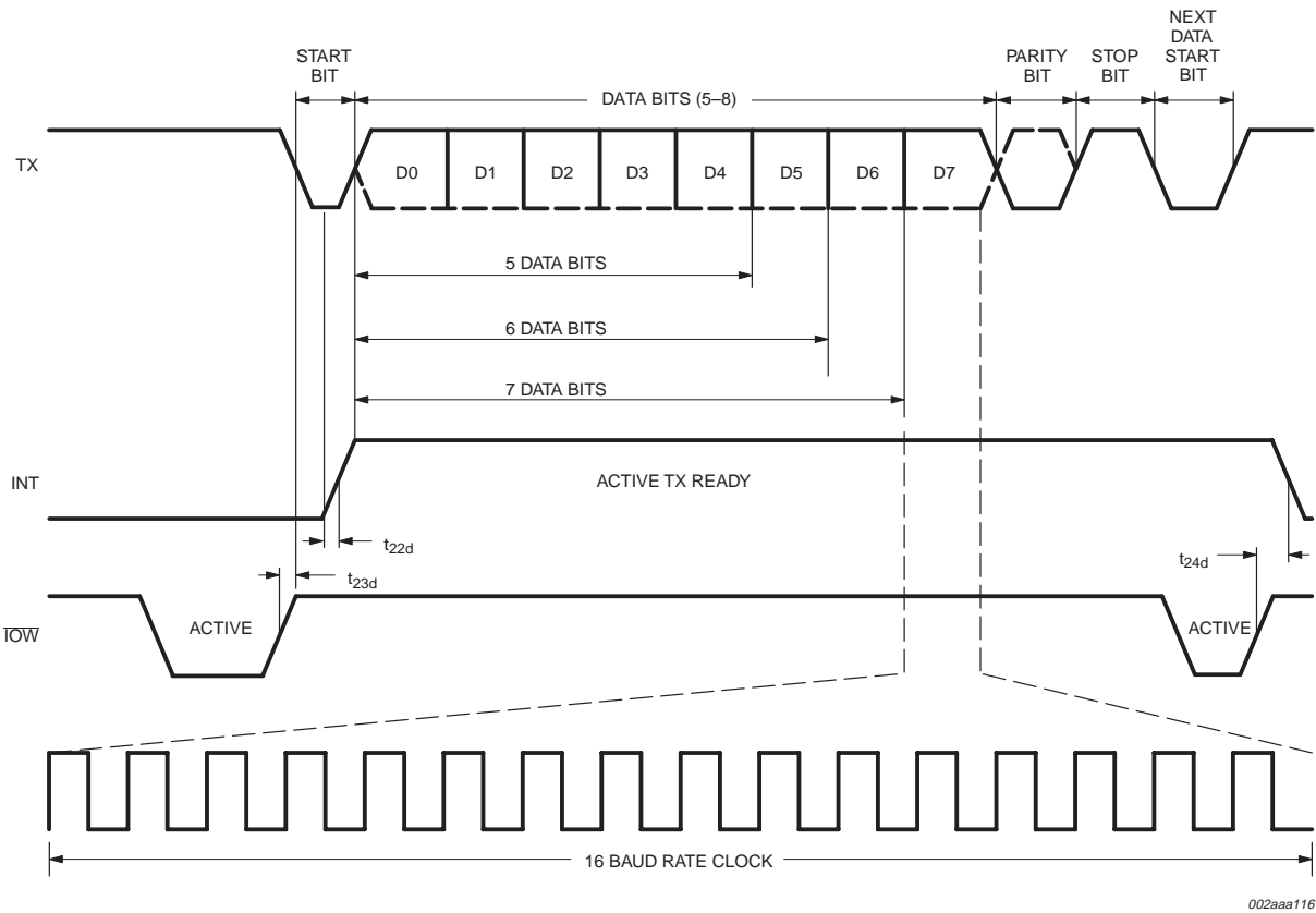
Fig 15. Transmit timing.
