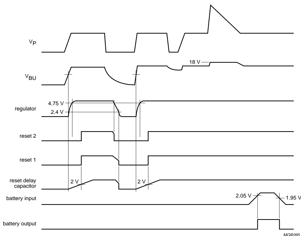
Fig.4 Timing diagrams.
