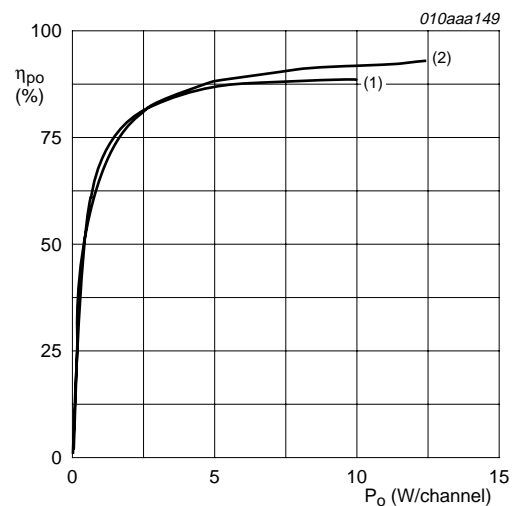
\eta_{po} = (2 \times P_o) / (2 \times P_o + P) (1) V_P = 17 \, \text{V} ; R_L = 2 \times 4 \, \Omega ; f_i = 1 \, \text{kHz} (2) V_P = 25 \, \text{V} ; R_L = 2 \times 8 \, \Omega ; f_i = 1 \, \text{kHz}
