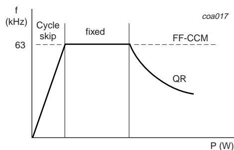
Fig 5. Multi mode and FF-CCM operation
