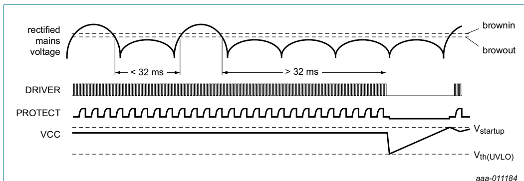
Fig 5. Mains detection
