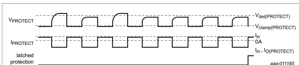
Fig 6. External overtemperature protection
