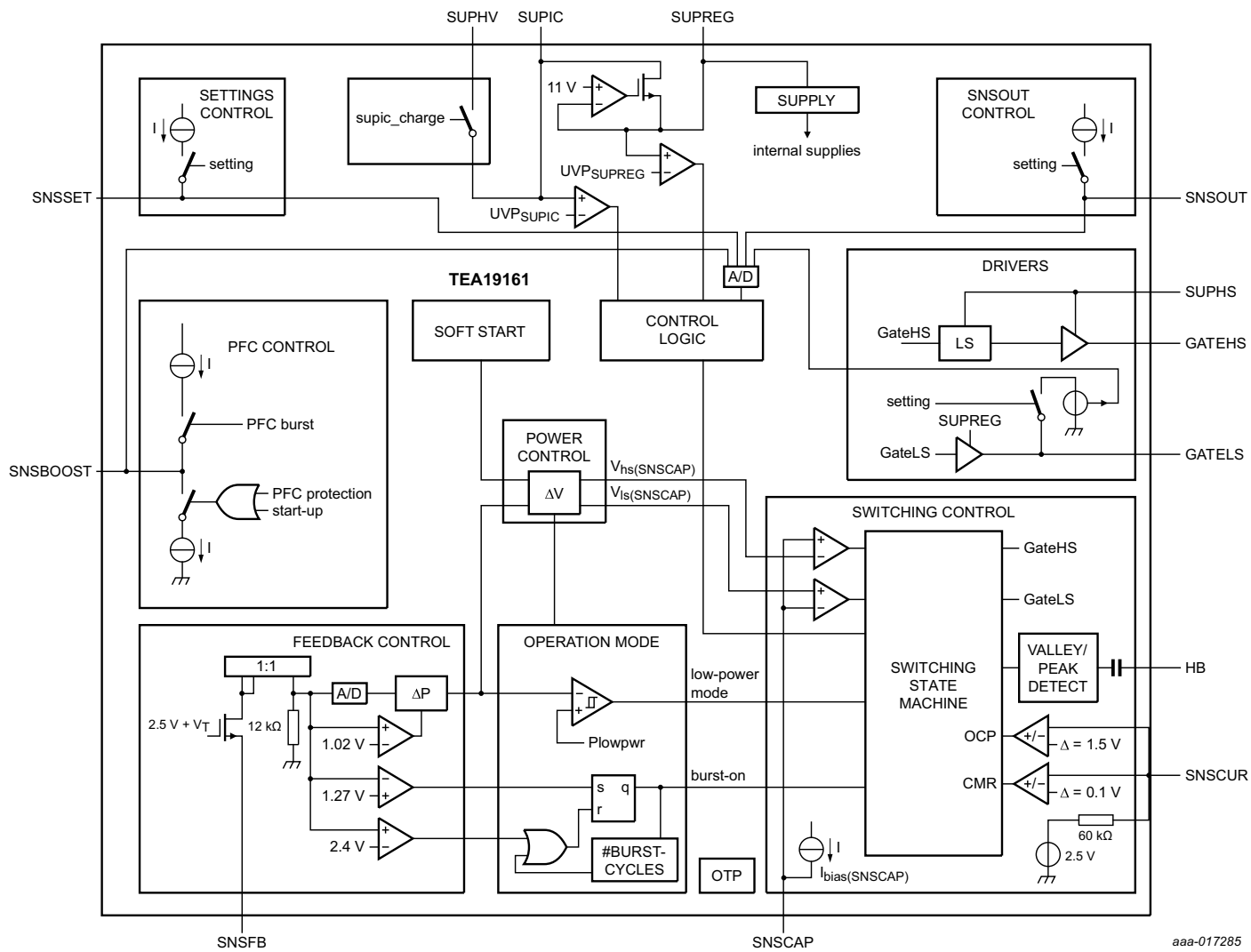
Fig 1. Block diagram
