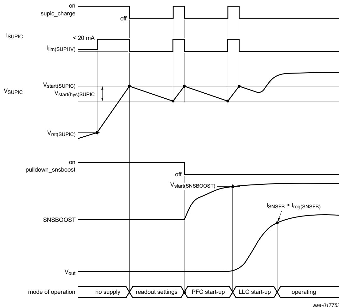
Fig 4. Start-up sequence and normal operation
