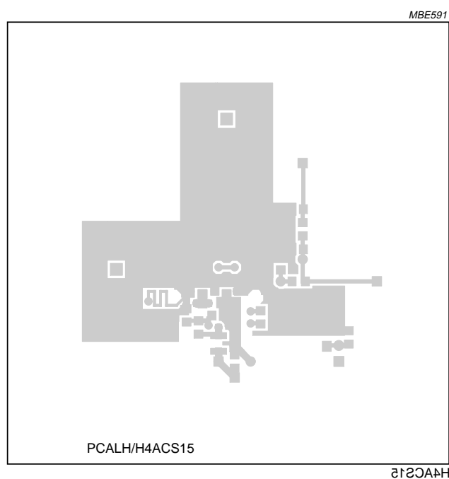
Fig.11 Layout bottom side.
