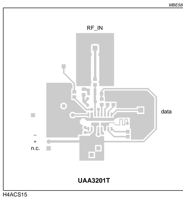
Fig.10 Layout top side.
