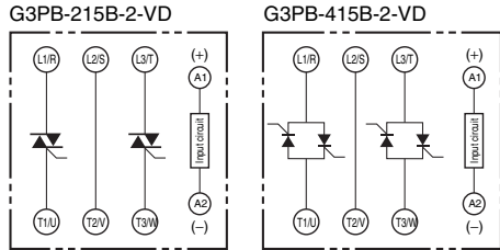
Terminal Arrangement/Internal Circuit Diagram
