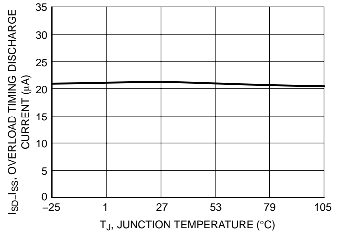
Figure 10. Overload Timing Discharge Current vs. Junction Temperature
