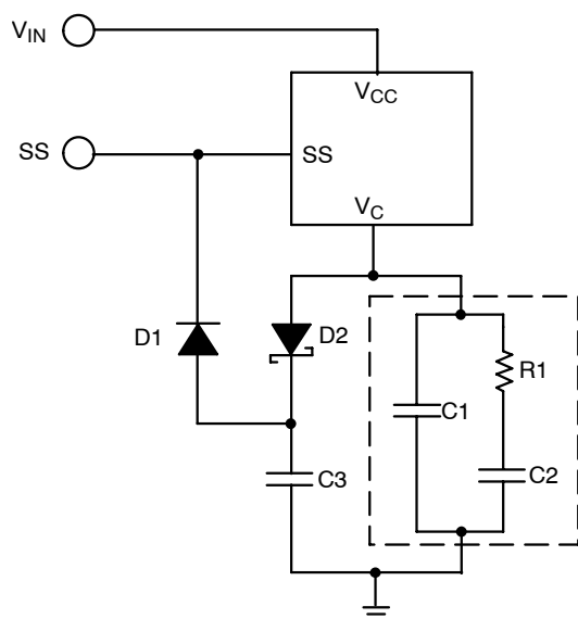
Figure 39. Soft-Start
