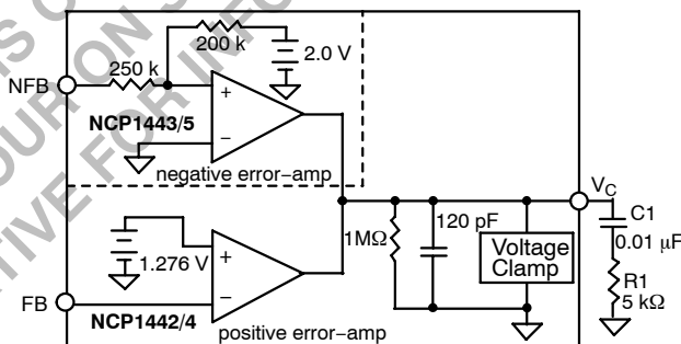
Figure 28. Error Amplifier Equivalent Circuit
