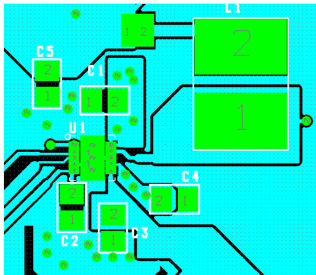
Figure 26. NCP1526 Board Layout
