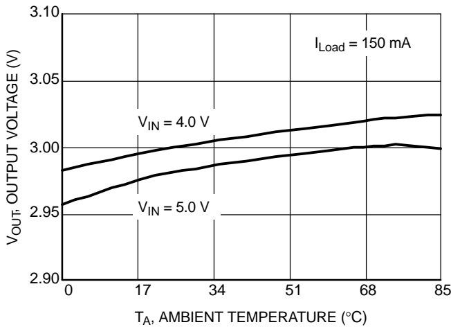
Figure 5. Output Voltage vs. Ambient Temperature ( V_{OUT} = 3.0 V)
