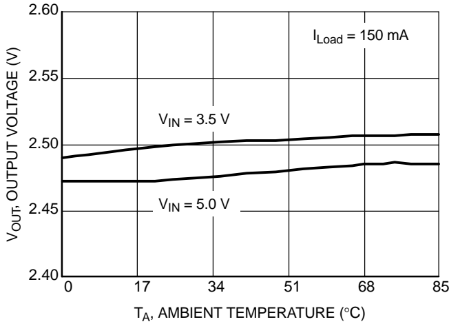
Figure 3. Output Voltage vs. Ambient Temperature ( V_{OUT} = 2.5 V)
