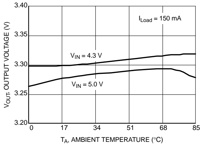
Figure 6. Output Voltage vs. Ambient Temperature ( V_{OUT} = 3.3 V)
