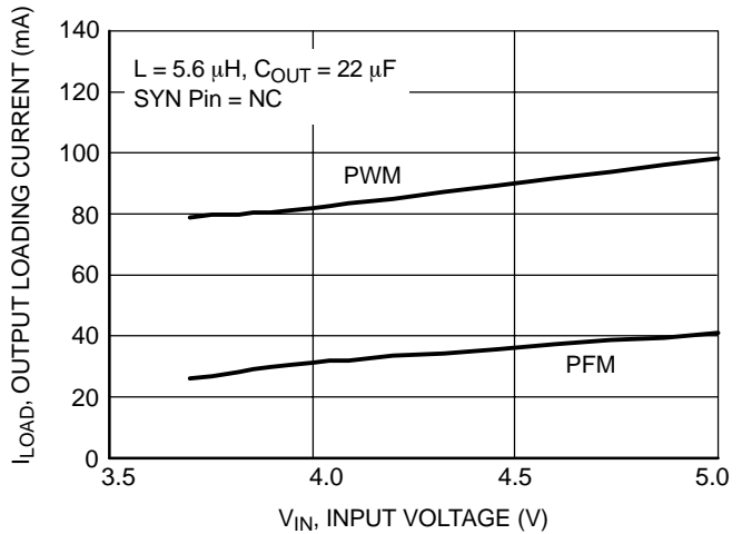
Figure 12. PWM/PFM Switchover Current Thresholds vs. Input Voltage ( V_{OUT} = 2.7\text{ V} )
