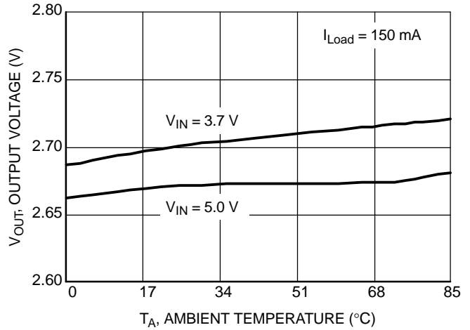
Figure 4. Output Voltage vs. Ambient Temperature ( V_{OUT} = 2.7 V)
