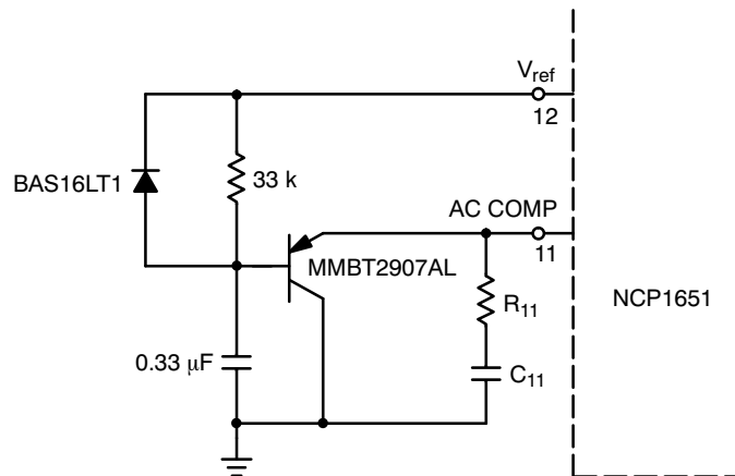
Figure 24. Soft-Start Circuit
