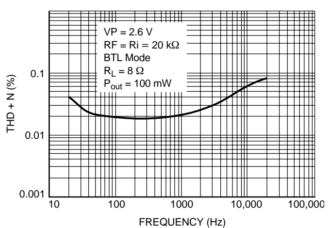
Figure 7. THD + N vs. Frequency (BTL Mode)
