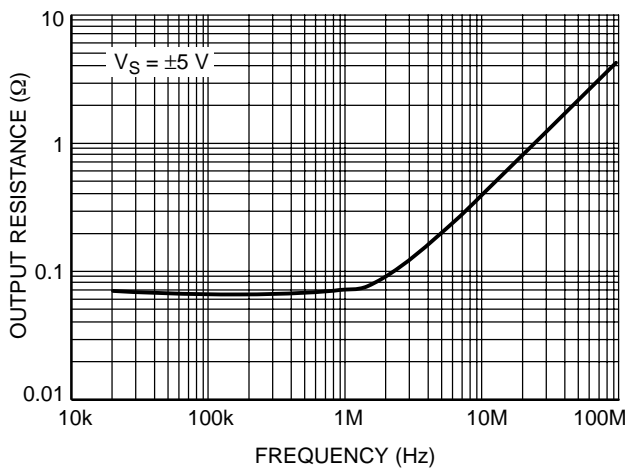
Figure 21. Closed-Loop Output Resistance vs. Frequency
