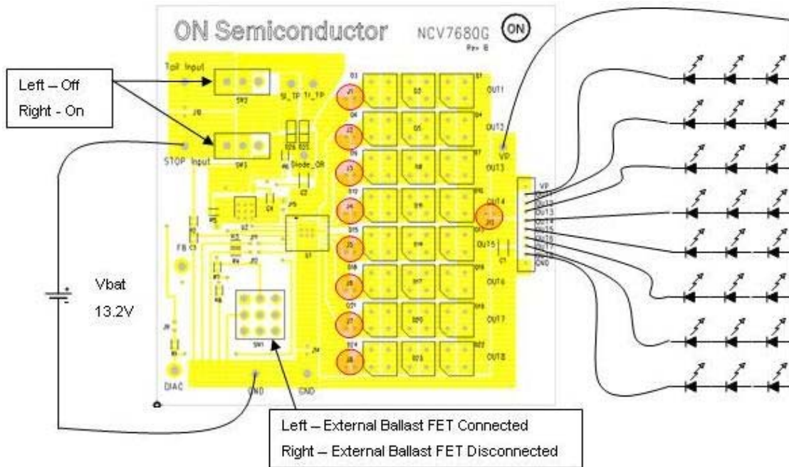
Figure 9. External LED's
