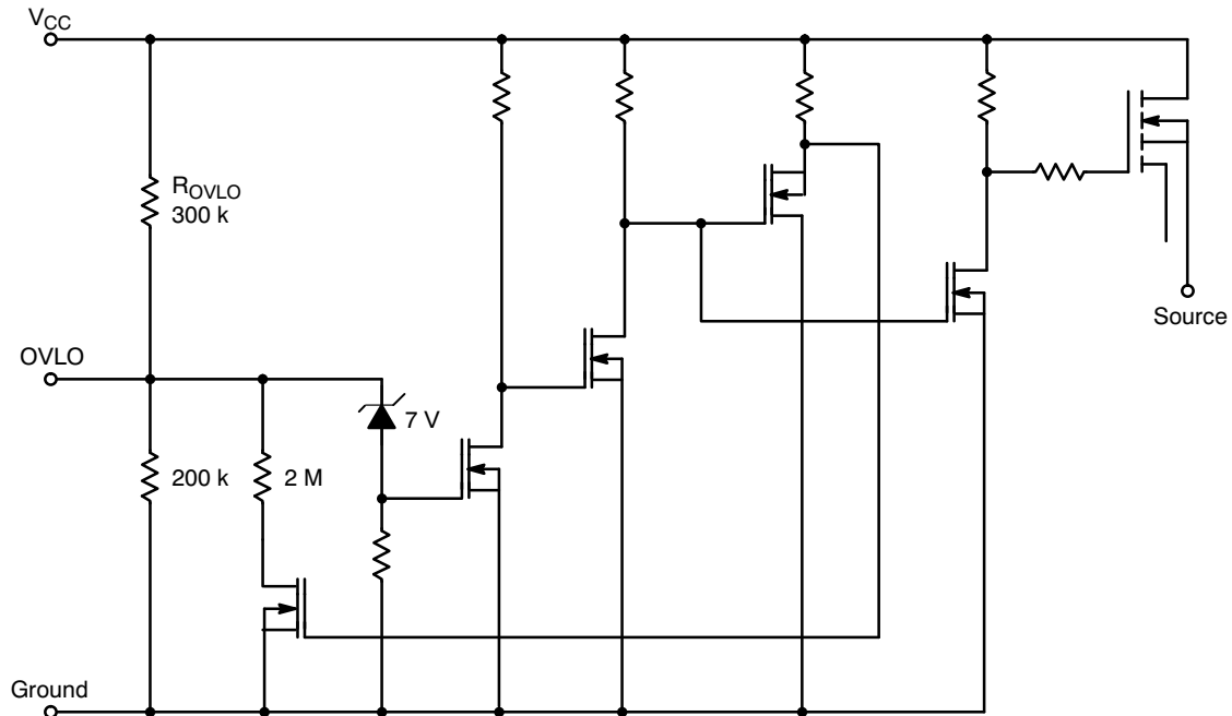
Figure 21. Equivalent Overvoltage Lockout Circuit
