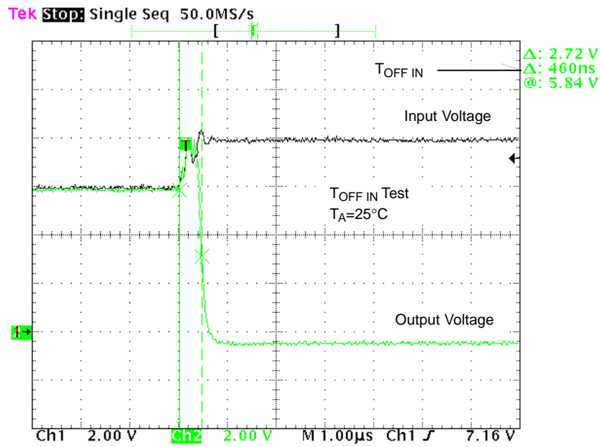
Figure 11. T_{\text{OFF IN}} Waveforms
