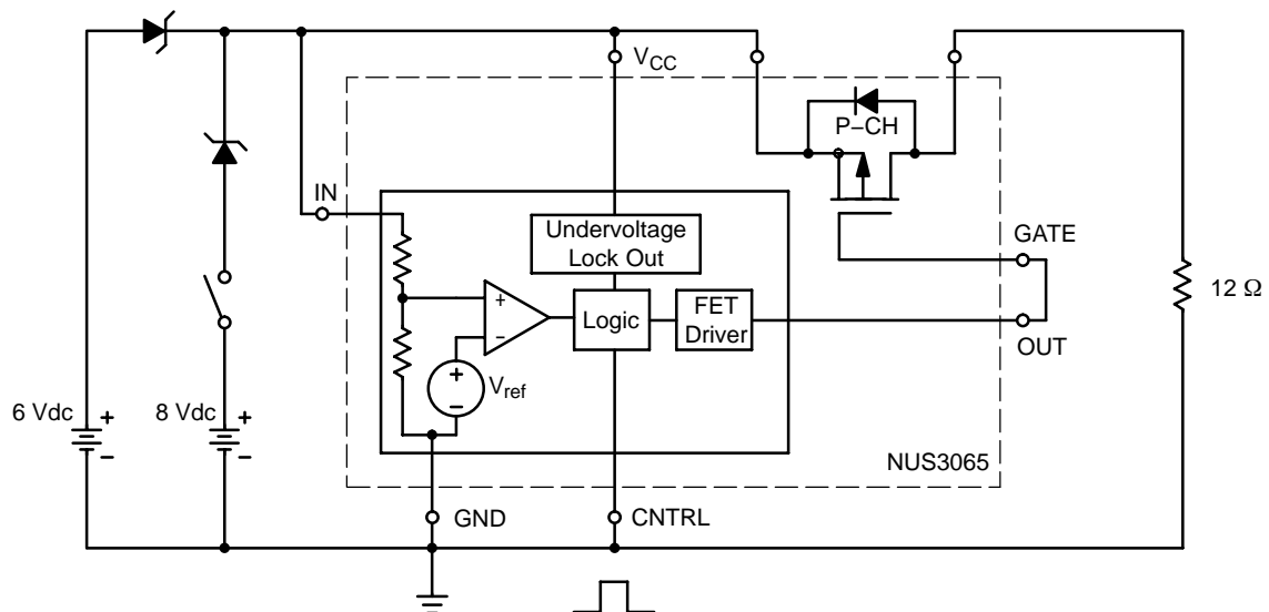
Figure 12. Test Circuit for T_{\text{ON CT}} and T_{\text{OFF CT}}
