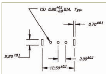
P.C. MOUNTING
