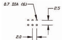
P.C. MOUNTING
