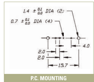
P.C. MOUNTING
