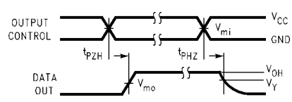
FIGURE 2. Waveforms (Input Pulse Characteristics; f=1MHz , t_r=t_f=3ns )
