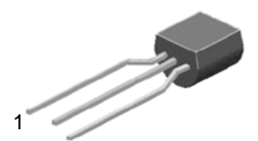
TO-92 1. Collector 2. Base 3. Emitter
