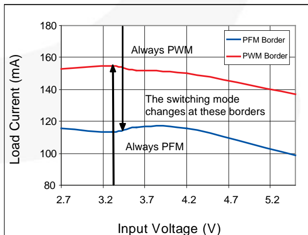
Figure 9. PFM / PWM Boundaries
