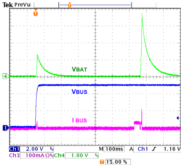
Figure 17. No Battery at V_{\text{BUS}} Power-up; FAN5400, FAN5403
