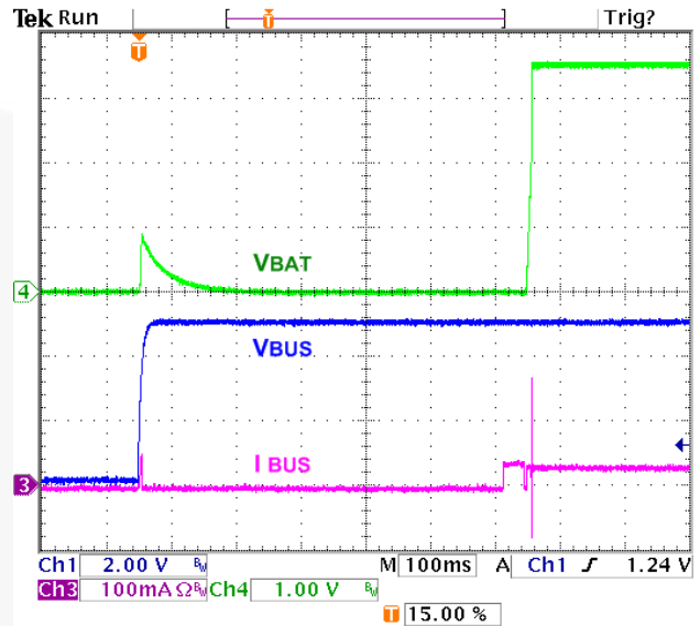
Figure 18. No Battery at V_{\text{BUS}} Power-up; FAN5402, FAN5405
