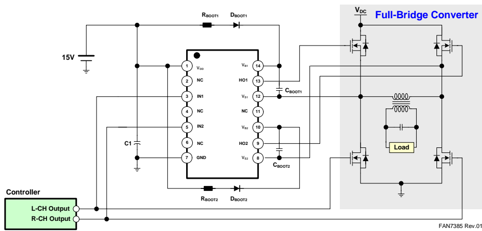
Figure 2. Full-Bridge Power Supply Application
