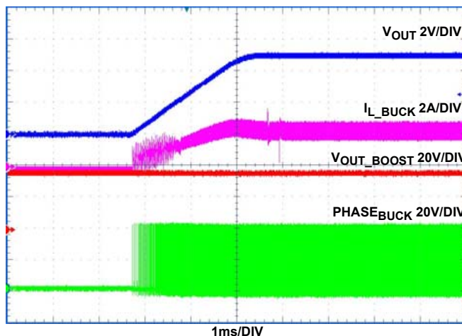
FIGURE 25. SOFT-START WITH 2\Omega LOAD ( V_{IN} = 36V )
