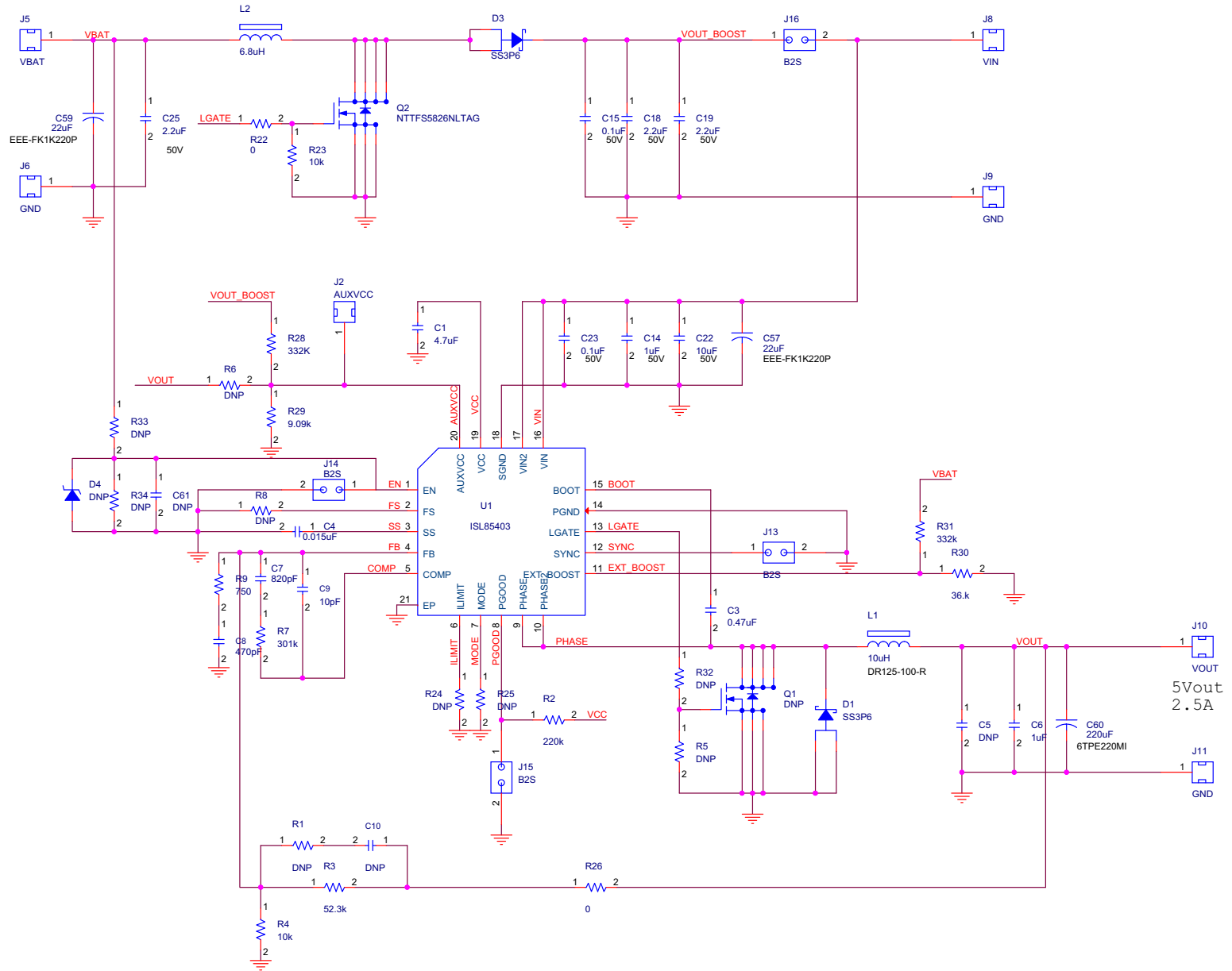
FIGURE 5. ISL85403EVAL1Z SCHEMATIC
