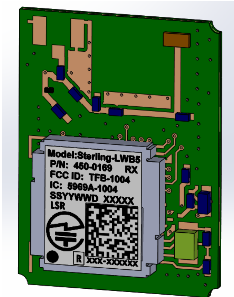
Figure 3 Sterling-LWB5 Chip Antenna Module (450-0169)
