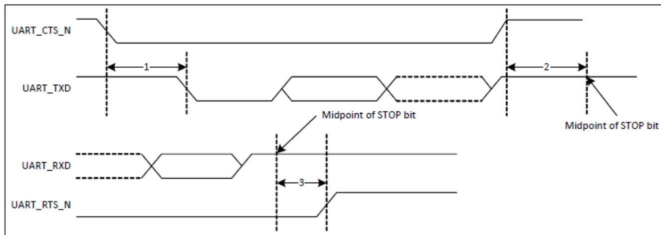
Figure 20 UART Timing
