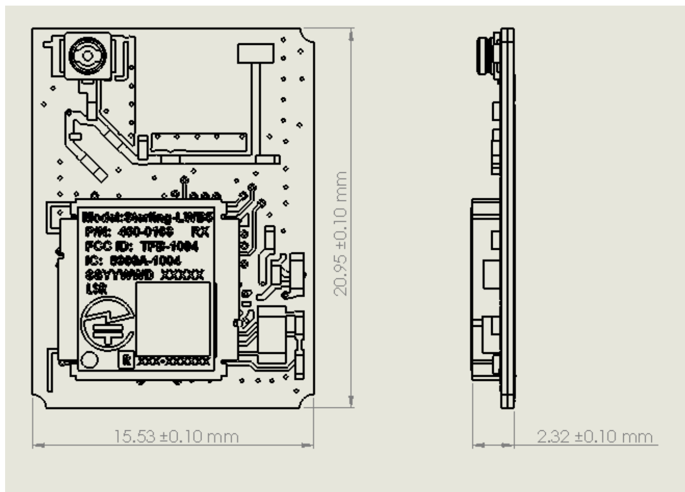
Figure 37 U.FL and Chip Antenna Mechanical Dimensions
