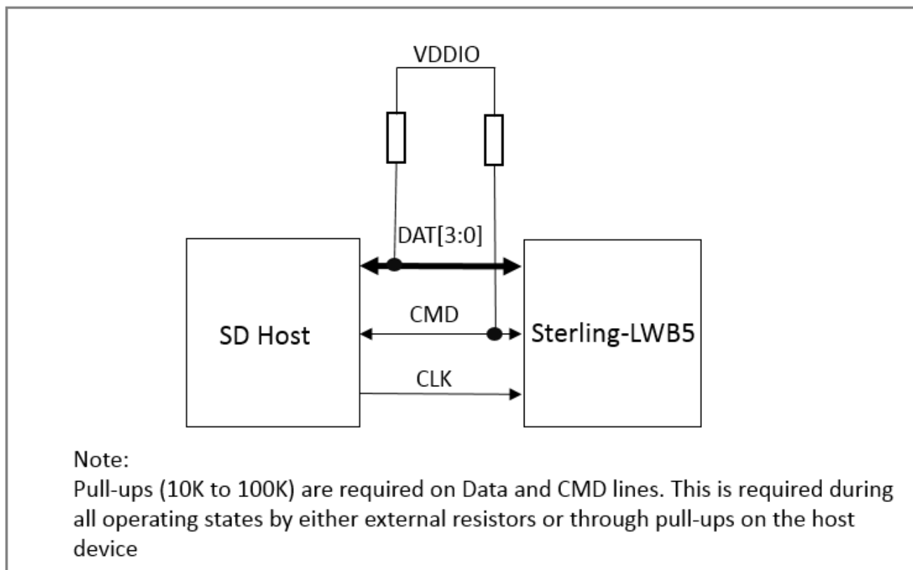
Figure 17 Signal Connections to SDIO Host (SD 4-Bit Mode)
