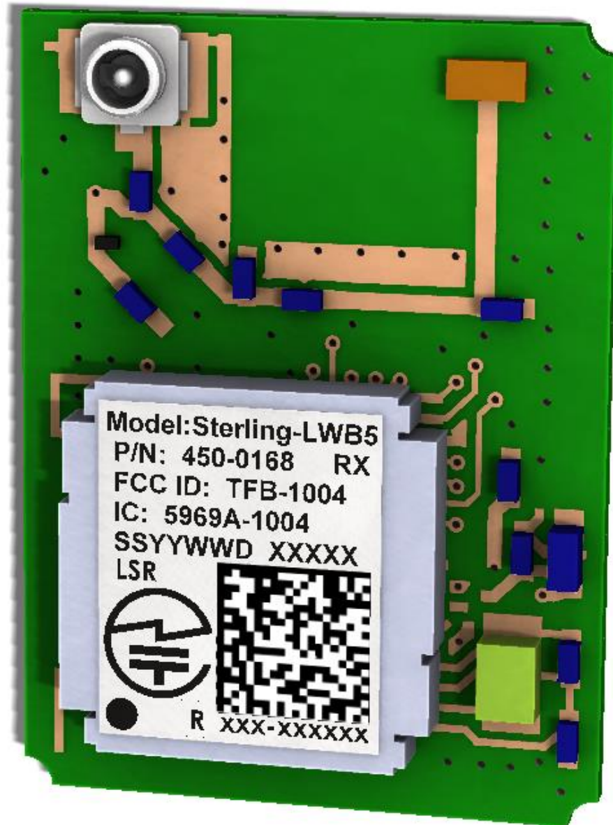
Figure 2 Sterling-LWB5 U.FL Module (450-0168)
