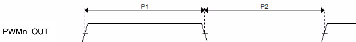
Figure 79. PWM Timing
