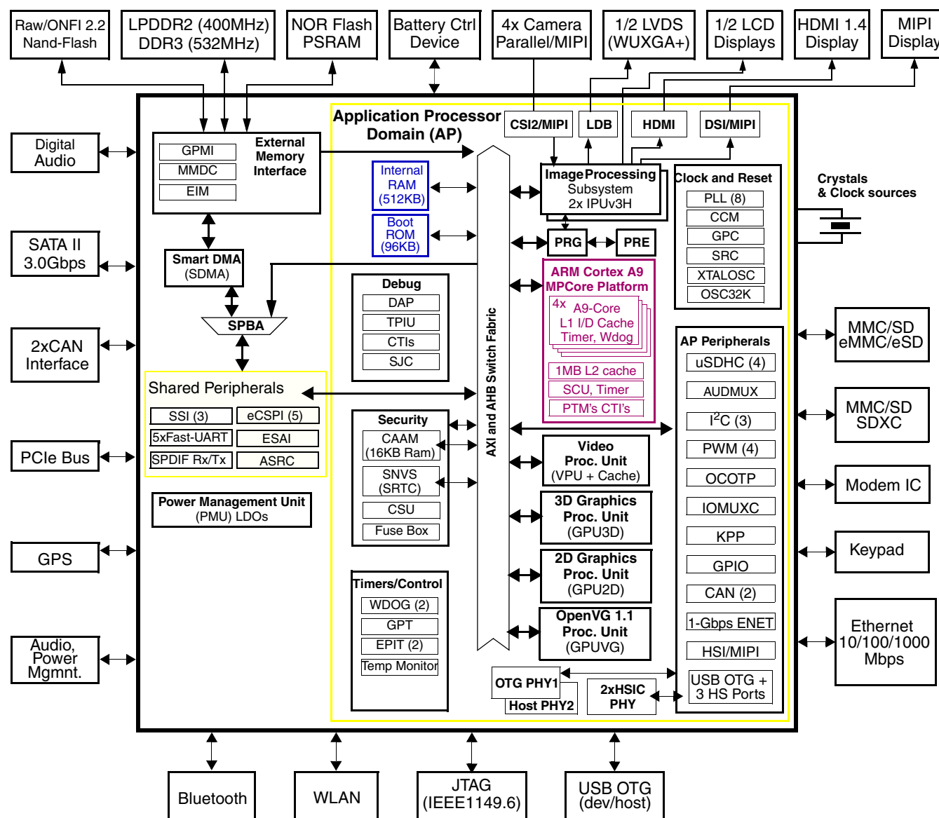
Figure 2. i.MX 6DualPlus/6QuadPlus Industrial Grade System Block Diagram
