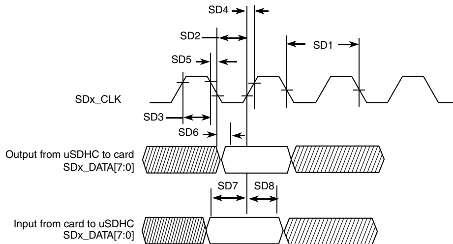
Figure 37. SD/eMMC4.3 Timing
