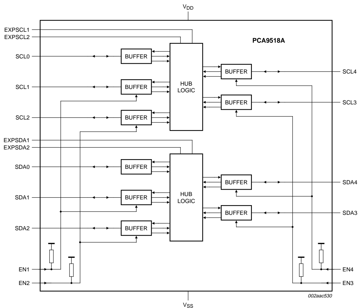
Fig 1. Block diagram of PCA9518A
