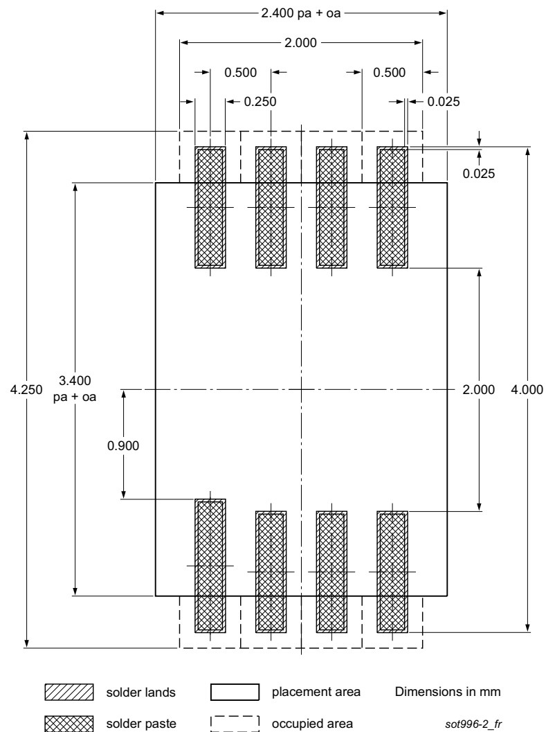
Fig 23. PCB footprint for SOT996-2 (XSON8); reflow soldering
