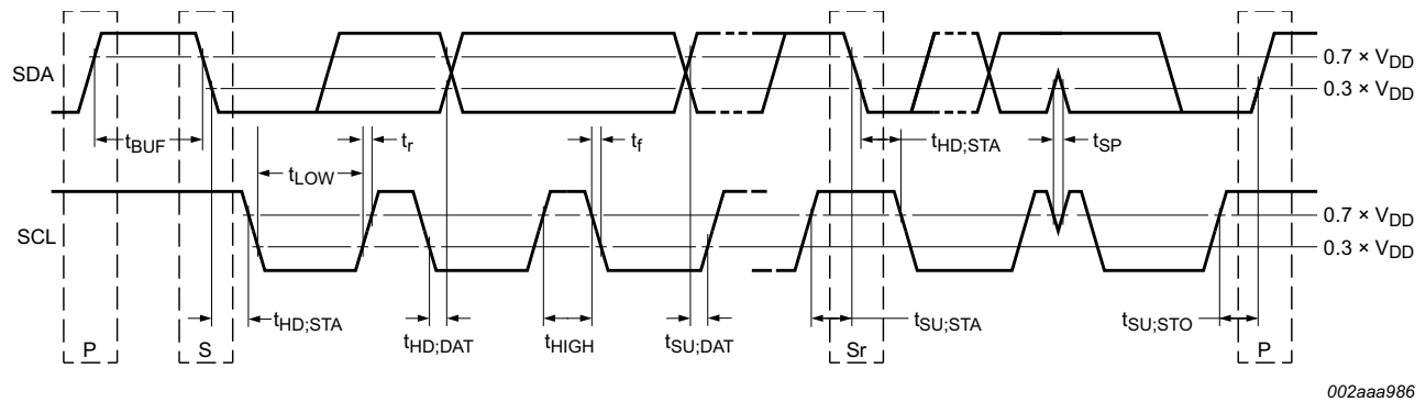
Fig 15. Definition of timing on the I 2 C-bus
