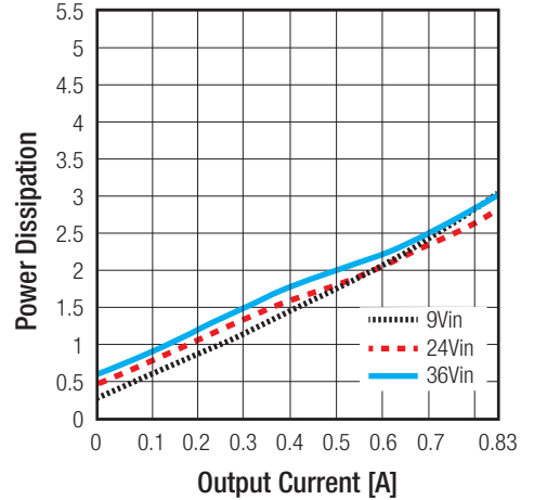
Power Dissipation vs Output Current
