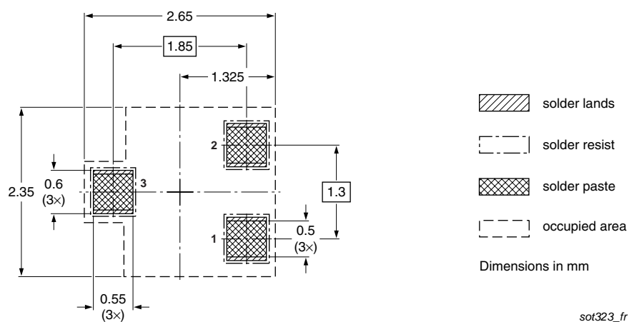
Fig 14. Reflow soldering footprint BAV99W (SOT323/SC-70)
