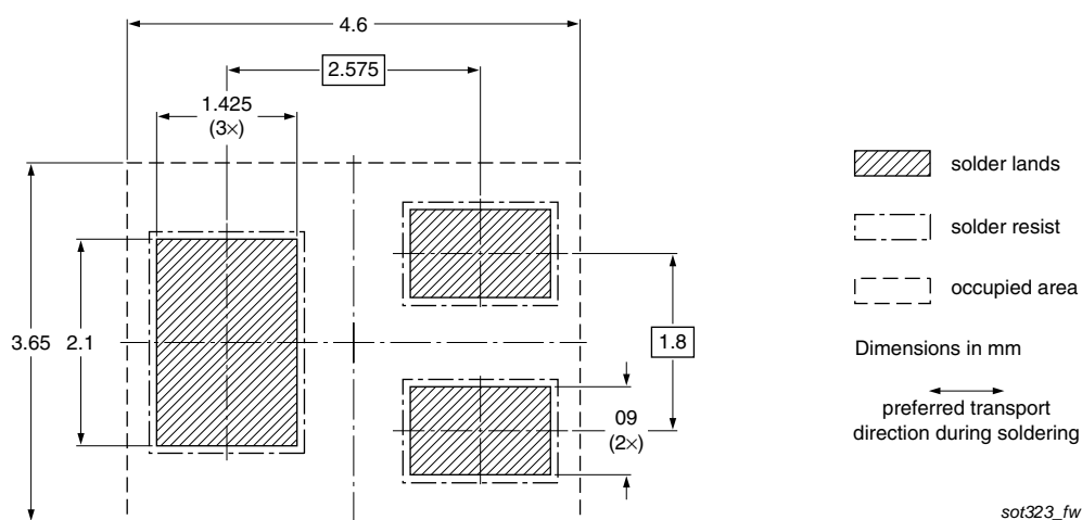
Fig 15. Wave soldering footprint BAV99W (SOT323/SC-70)
