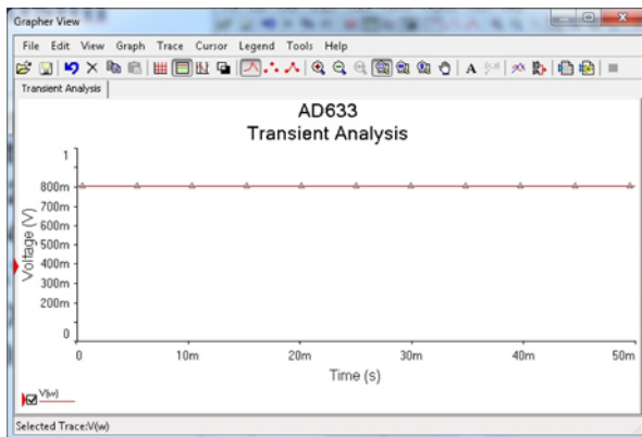
Figure 25. Circuit to Multiply Two Integers Response Graph Displayed in Multisim (2\text{ V} \times 4\text{ V})/10\text{ V} = 0.8\text{ V}
