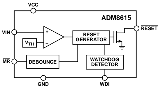
Figure 26. ADM8615 Functional Block Diagram
