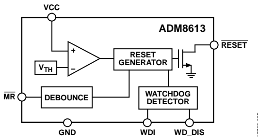
Figure 25. ADM8613 Functional Block Diagram
