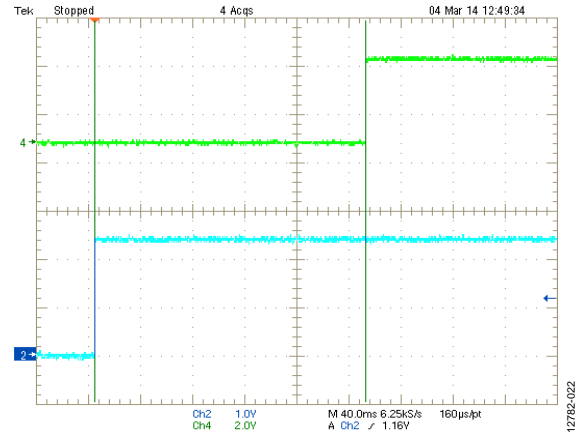
Figure 22. \overline{\text{RESET}} Timeout Delay With V CC and V IN Rising
