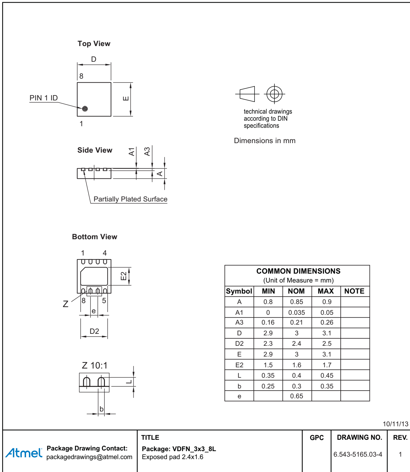
Figure 11-1. DFN8
