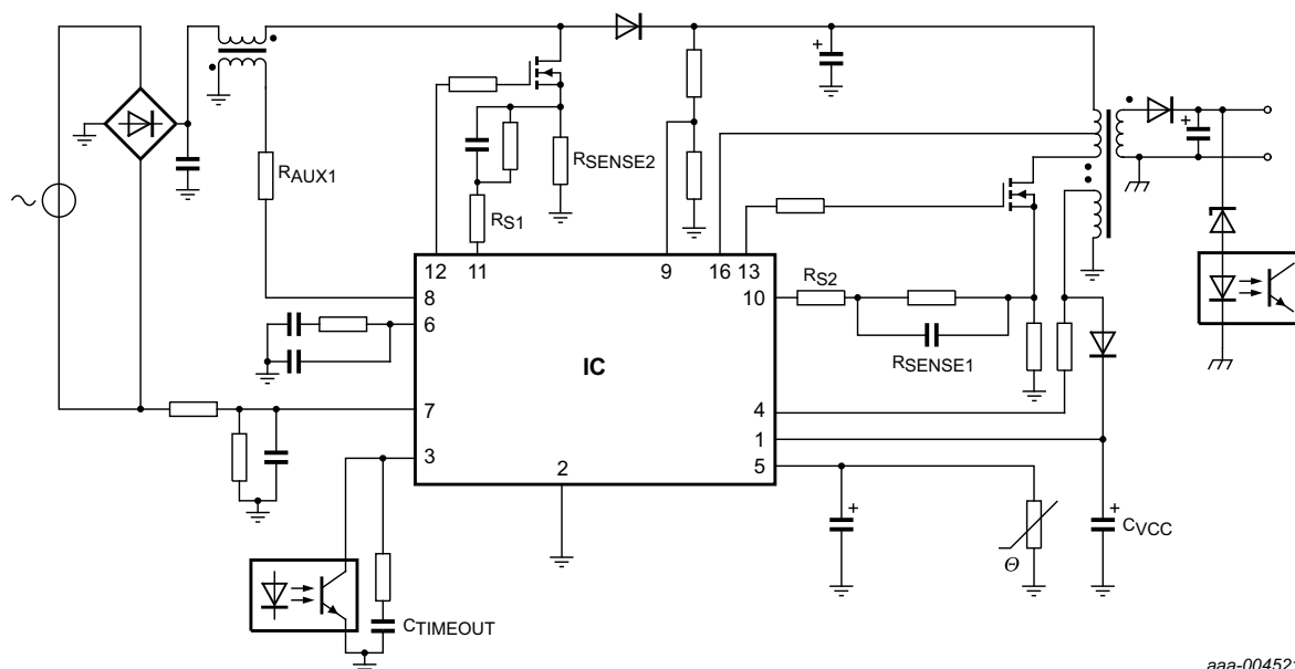
Fig 16. Typical application diagram for the TEA1751T
