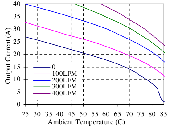
Figure 14. QHS40ZB (1.8V) Derating Curves
