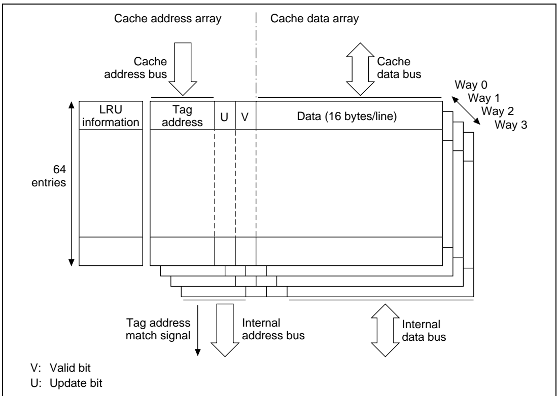
Figure 8.1 Cache Configuration
