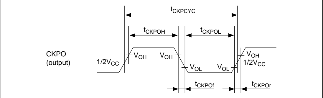
Figure 21.4 CKPO Clock Output Timing
