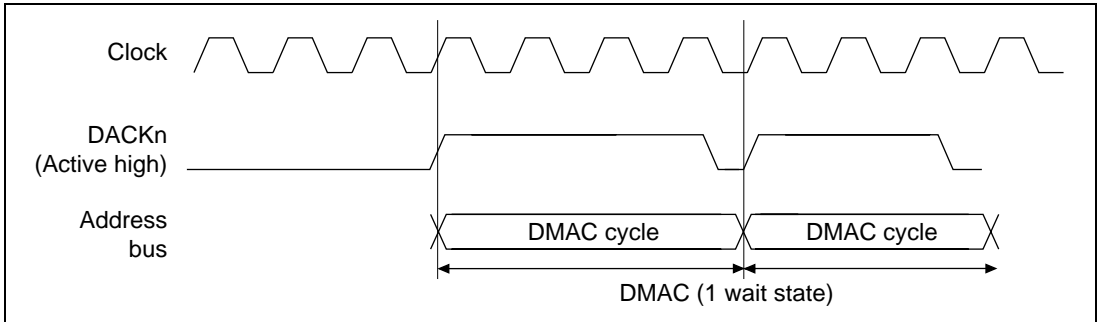
Figure 11.32 DACKn Output in Nibble Accesses of Burst ROM
