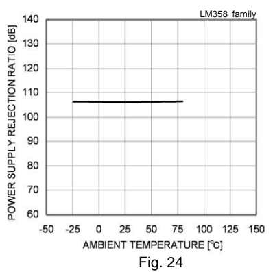
Fig. 24 Power Supply Rejection Ratio – Ambient Temperature
