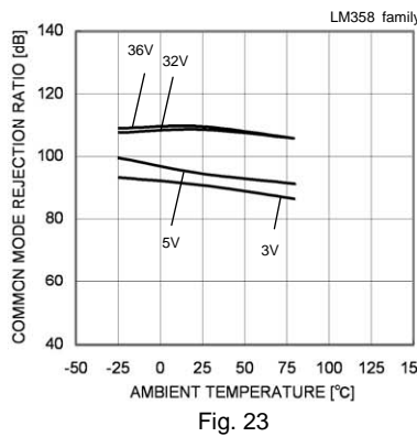
Fig. 23 Common Mode Rejection Ratio – Ambient Temperature
