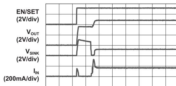
Turn On to 2X Mode ( V_{IN} = 3.6V ; 20.5mA/ch)
