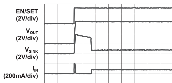
Turn On to 1X Mode ( V_{IN} = 4.2V ; 20.5mA/ch)
