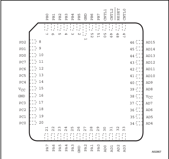
Figure 2. PLCC Connections
