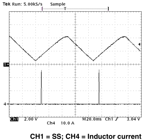
Figure 8. Hiccup Mode
