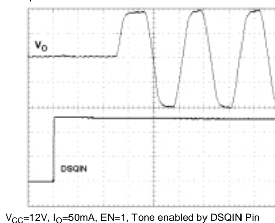
Figure 28 : DSQIN Tone Enable Transient Response
