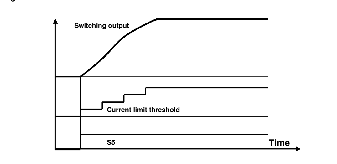
Figure 35. Soft-start waveforms
