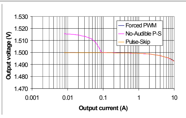
Figure 10. VDDQ load regulation, 1.5 V, Vin = 12 V
