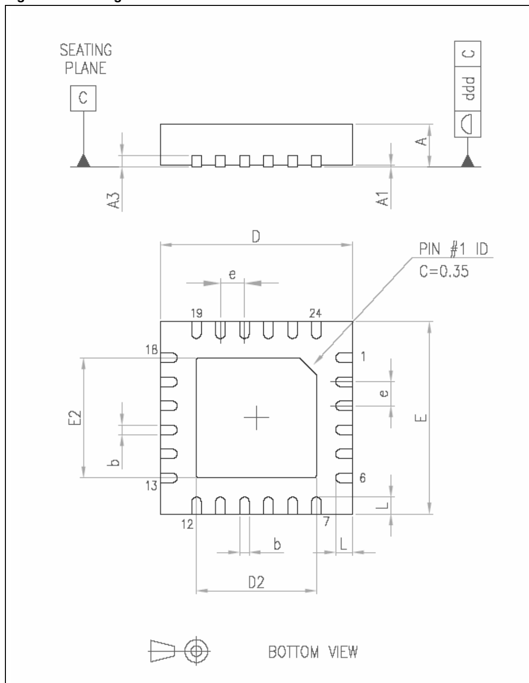
Figure 42. Package dimensions
