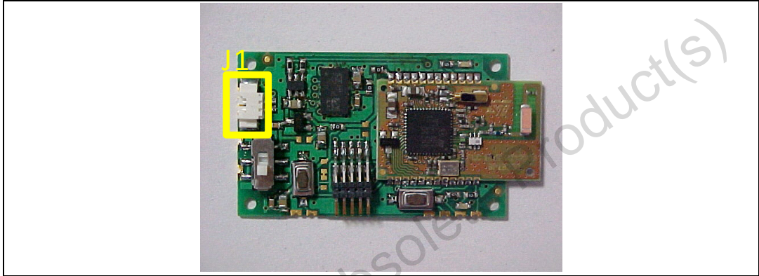
Figure 3. J1 connector
