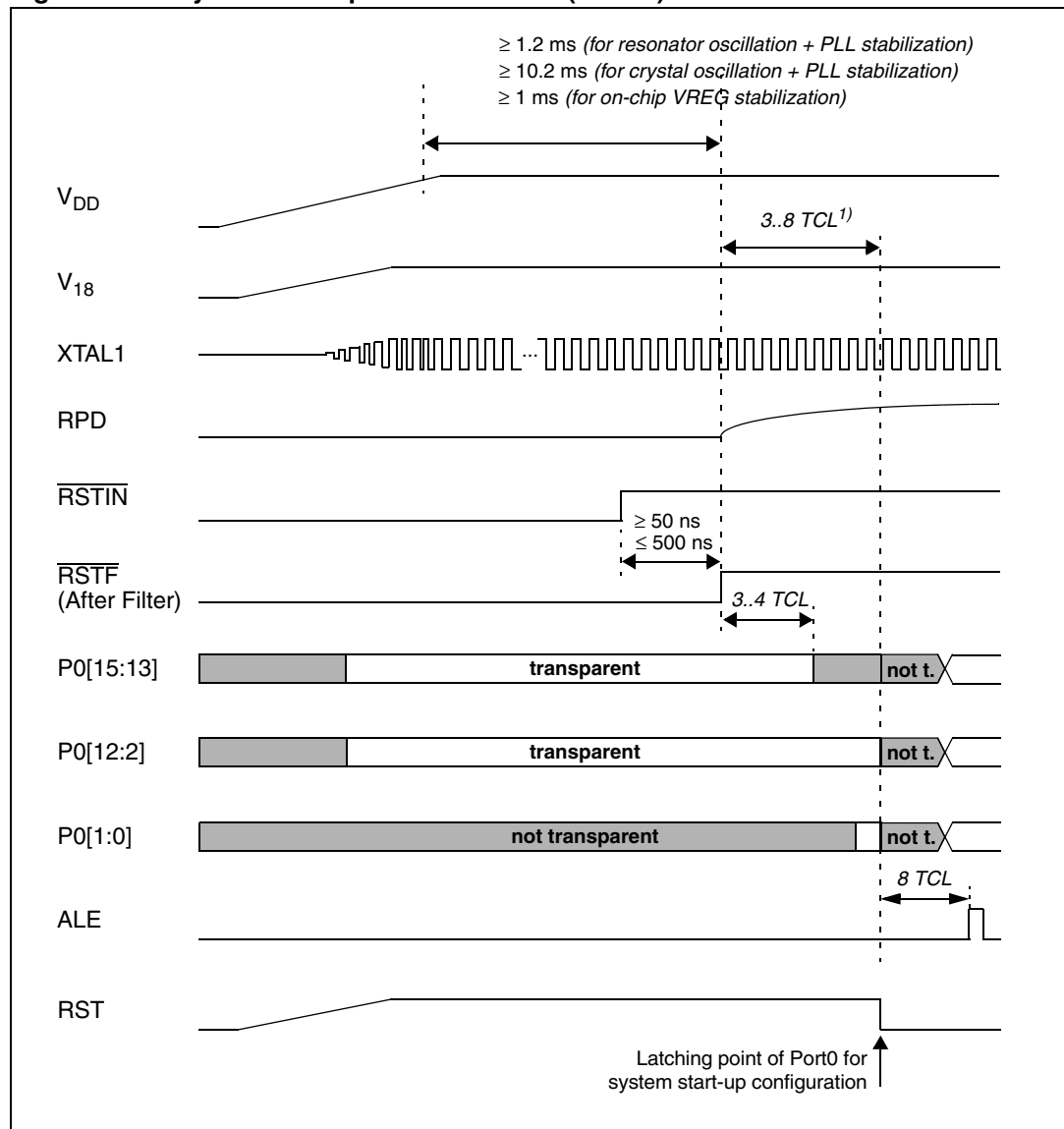
Figure 16. Asynchronous power-on RESET ( \overline{\text{EA}} = 0 )
