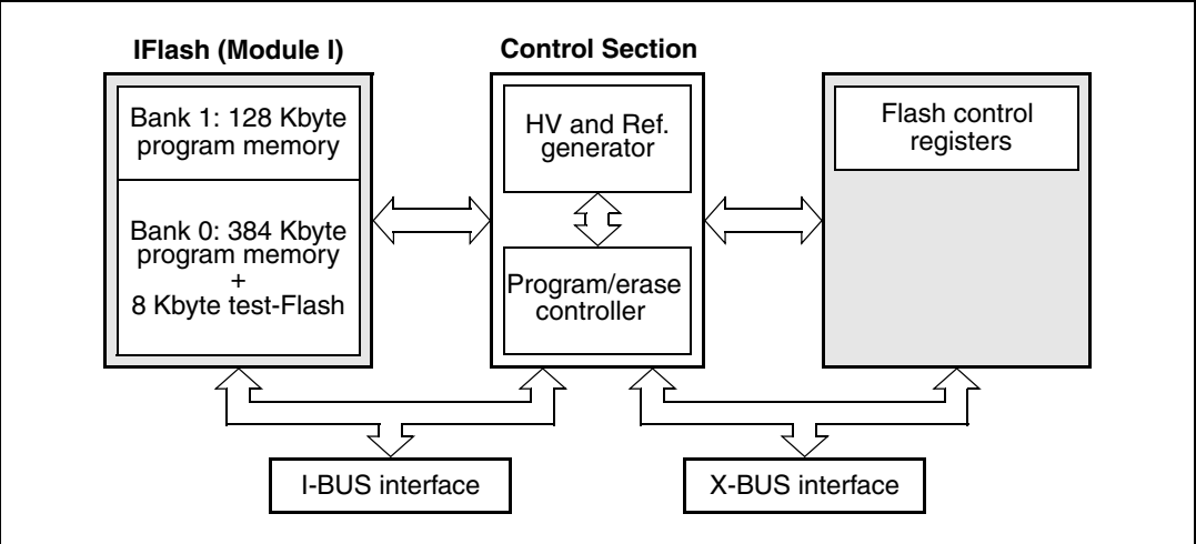
Figure 4. Flash structure
