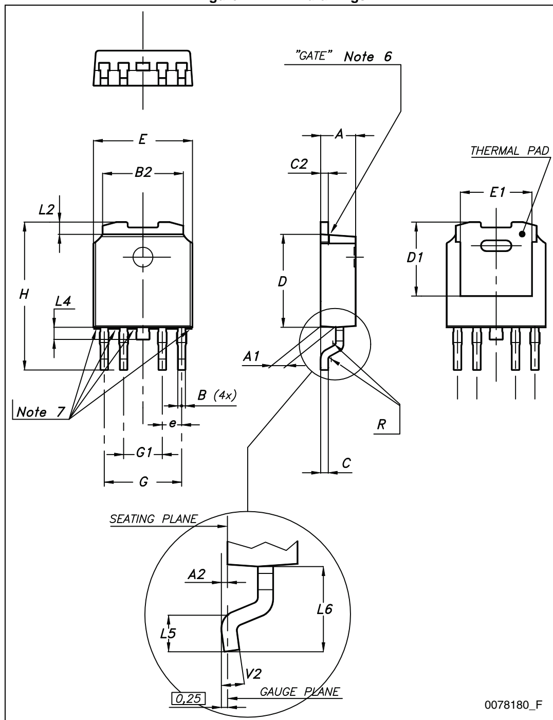
Figure 24. PPAK drawings
