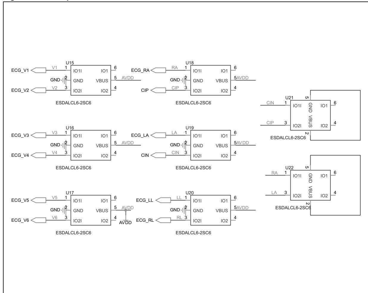
Figure 3. ESD protection
