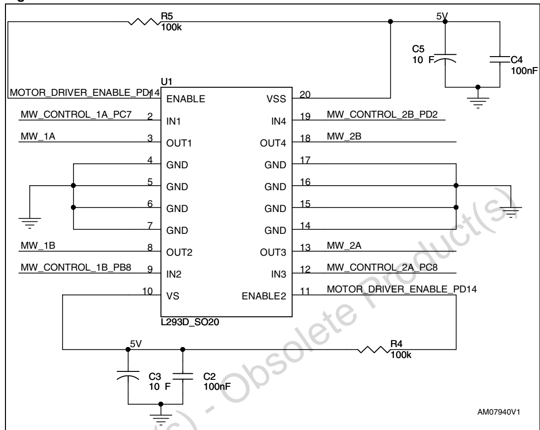
Figure 3. Motor driver
